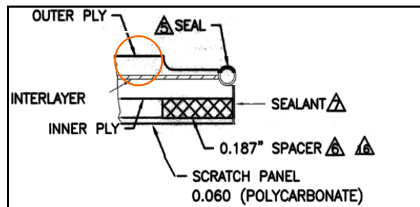
CROSS SECTION OF PERKINS LAMINATED WINDOW
